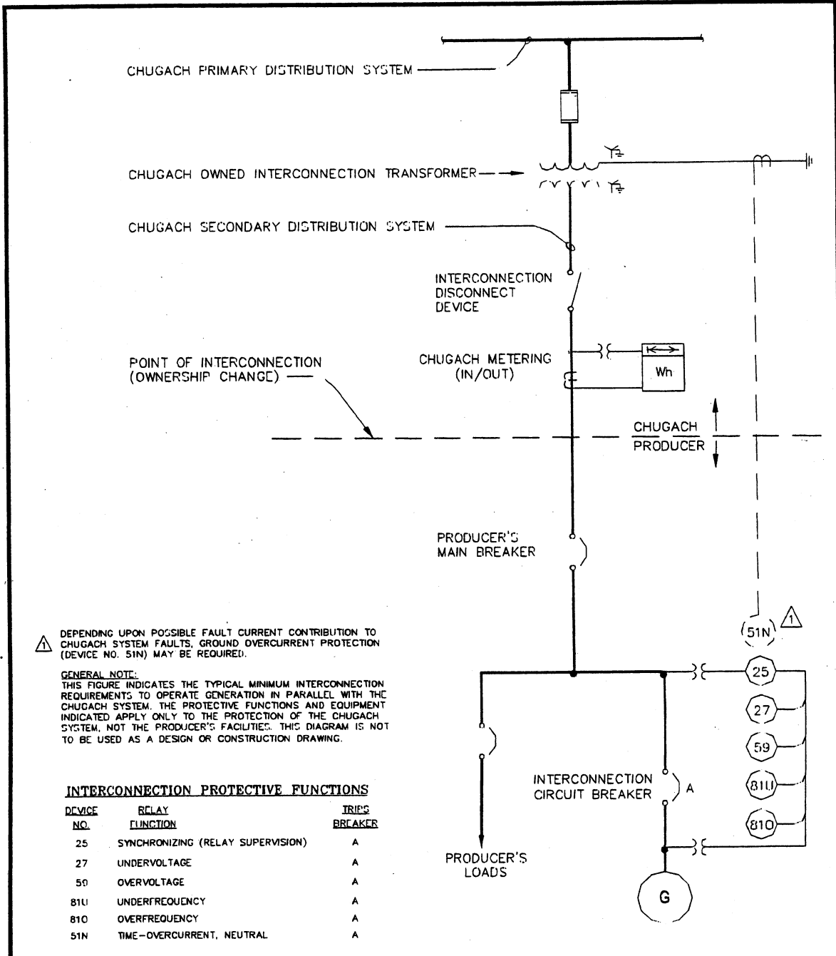
FIGURE B-1 TYPICAL SECONDARY SYSTEM INTERCONNECTION CLASS B FACILITIES (10KVA TO 100KVA) DRAWING NUMBER: NUG_FIGB-1 SHEET 1 OF 1
