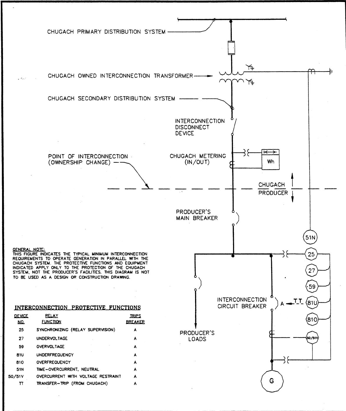
FIGURE D-1 TYPICAL SECONDARY SYSTEM INTERCONNECTION CLASS D FACILITIES (1000 KVA TO 5000KVA)
