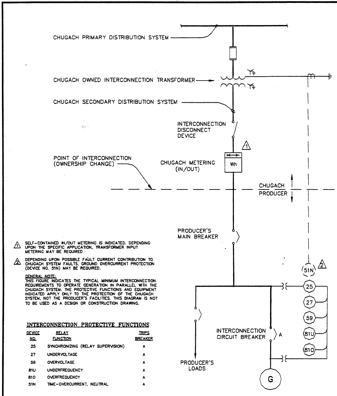
FIGURE A-1 TYPICAL SECONDARY SYSTEM INTERCONNECTION CLASS A FACILITIES (10KVA AND LESS)
